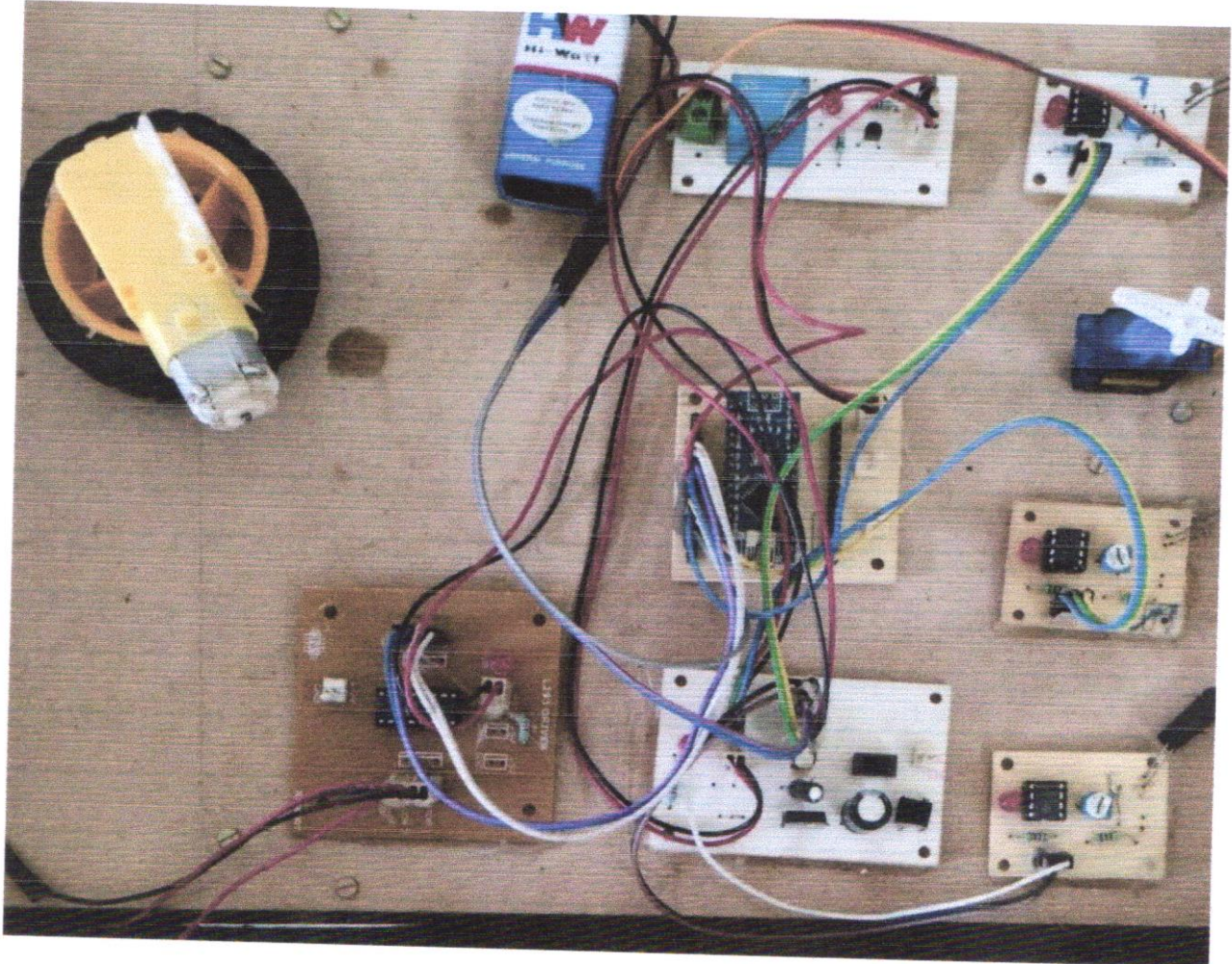
FIRE FIGHTING ROBOT
